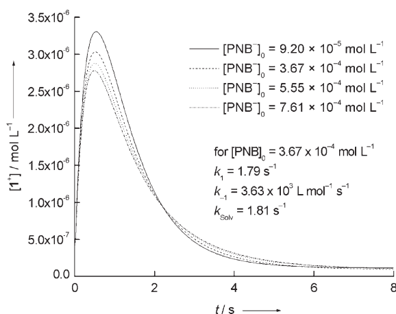
Figure 3. Formation and consumption of the blue 1^+ ion (monitored photometrically at 612 nm) during the solvolysis of 1-PNB ( 1.04 \times 10^{-5} \text{ mol L}^{-1} ) in 60% aqueous acetone in the presence of different amounts of n\text{Bu}_4\text{N}^+\text{PNB}^- at 25^\circ\text{C} .
