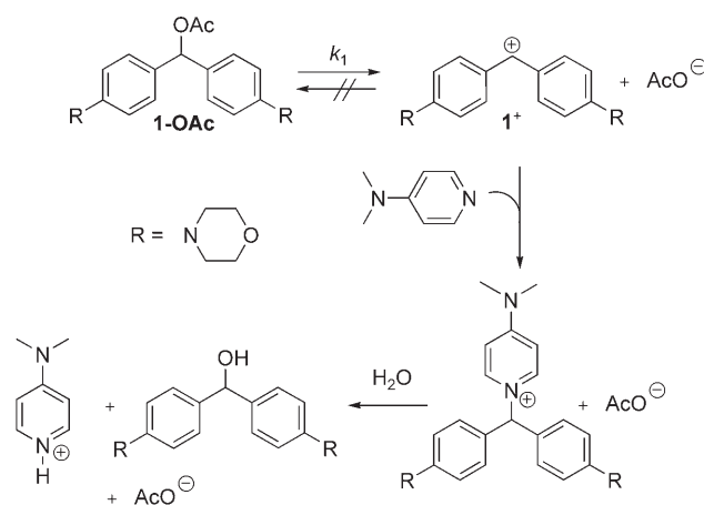
Scheme 3. Trapping of the intermediate benzhydrylium ions by DMAP.
