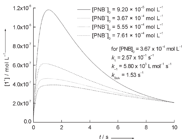
Figure 2. Formation and consumption of the blue 1^+ ion (monitored photometrically at 612 nm) during the solvolysis of 1-PNB ( 1.04 \times 10^{-5} \text{ mol L}^{-1} ) in 80% aqueous acetone in the presence of different amounts of n\text{Bu}_4\text{N}^+\text{PNB}^- at 25^\circ\text{C} .
