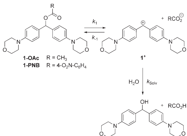
Scheme 2. Solvolysis reaction of 4,4'-bis(morpholino)benzhydryl carboxylates in aqueous acetone or acetonitrile.
