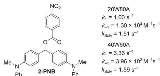
Figure 4. Rate constants for the solvolysis of the 2-PNB ( 9.48 \times 10^{-4} \text{ mol L}^{-1} ) in 80% and 60% aqueous acetone in the presence of 3.67 \times 10^{-4} \text{ mol L}^{-1} n\text{Bu}_4\text{N}^+\text{PNB}^- .
