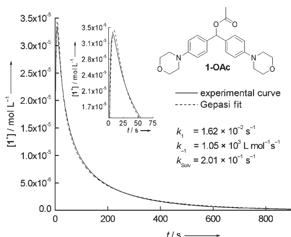
Figure 1. Formation and consumption of the blue 1^+ ion (monitored photometrically at 612 nm) during the solvolysis of 1-OAc ( 1.09 \text{ mmol L}^{-1} ) in 80% aqueous acetonitrile in the presence of (i\text{Pr})_2\text{NMe} ( 5.24 \text{ mmol L}^{-1} ) at 25^\circ\text{C} .
